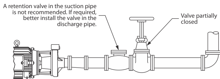
Figure 5 Positive suction.
